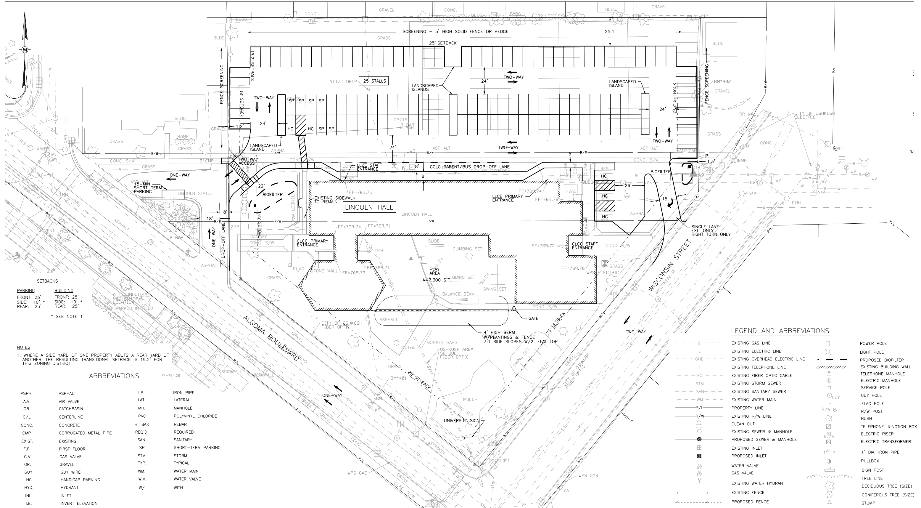
CONCEPTUAL SITE PLAN APPENDIX B-1
